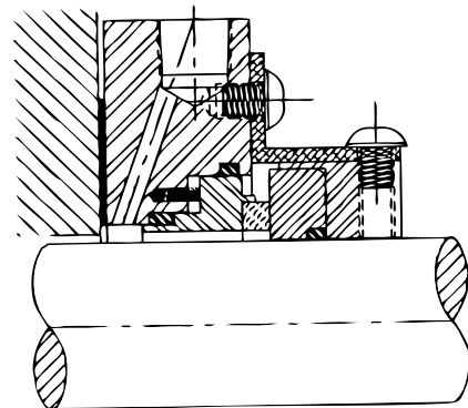
Style 20 — Single seal
